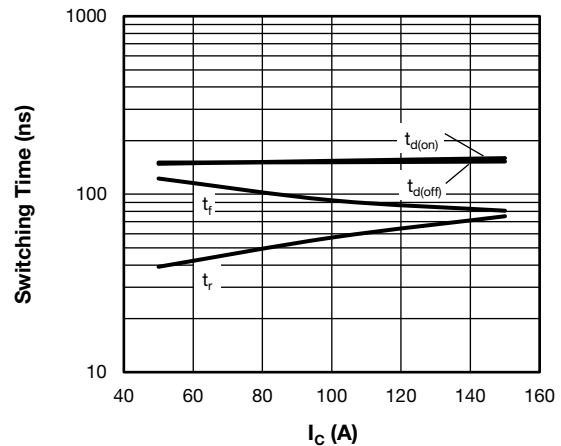
Fig. 26 - Switching Time vs. I_C (Typical Q2 - Q3 Trench IGBT Switching Time vs. I_C (with D2 - D3 Antiparallel Diode)), T_J = 125\text{ }^\circ\text{C} , V_{CC} = 325\text{ V} , R_g = 4.7\text{ }\Omega , V_{GE} = \pm 15\text{ V} , L = 500\text{ }\mu\text{H}
