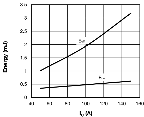
Fig. 25 - Energy Loss vs. I_C (Typical Q2 - Q3 Trench IGBT Energy Loss vs. I_C (with D2 - D3 Antiparallel Diode)), T_J = 125\text{ }^\circ\text{C} , V_{CC} = 325\text{ V} , R_g = 4.7\text{ }\Omega , V_{GE} = \pm 15\text{ V} , L = 500\text{ }\mu\text{H}
